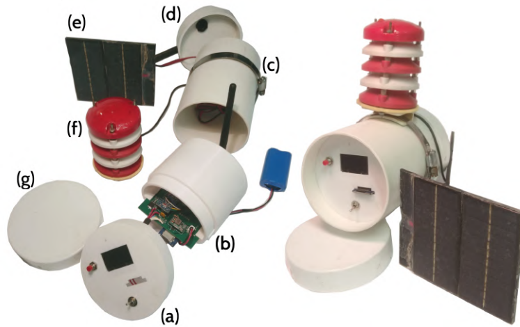
Figure C.16: Exploded view of the housing components of the IoT device: (a) Front of the device containing monitor button, ON/OFF switch, SD and Oled display (3D-printed part). (b) support for datalogger board, batteries and wireless module. (c) Four-inch PVC pipe. (d) and (g) Back and front cover. (e) Solar panel. (f) Relative humidity and air temperature sensor shield. On the right-hand side, all assembled housing parts.
