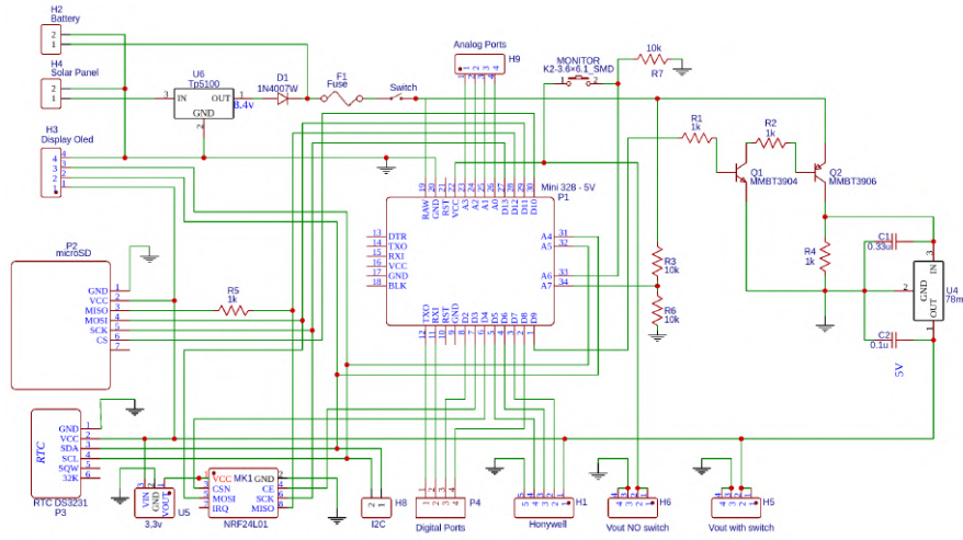
Figure C.15: Schematic diagram showing connectivity between different components of the IoT device.
