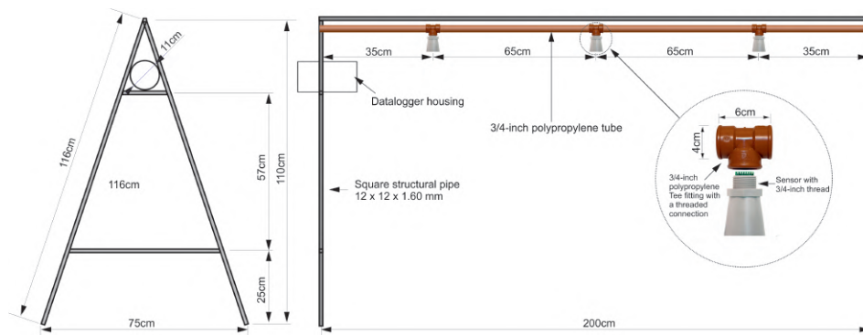
Figure D.11: Design of the crop growth monitoring station
