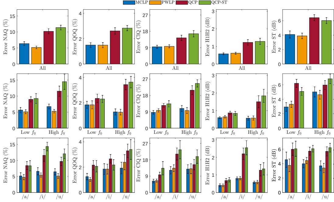
Figure 5: Bar plots of the estimation error for parameters NAQ, QOQ, ClQ, H1H2, and ST for the synthetic signals from repository II (with the 95% confidence intervals) for different voice inverse filtering methods. The errors are shown according to: all signals (top row), f_0 ranges (middle row), and vowel sounds (bottom row).
