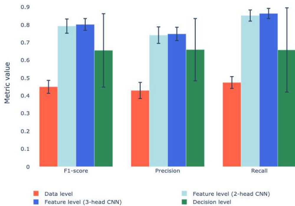
Figure 7: Comparison of the results obtained by different fusion levels based on the overalls F1-score, precision and recall.
