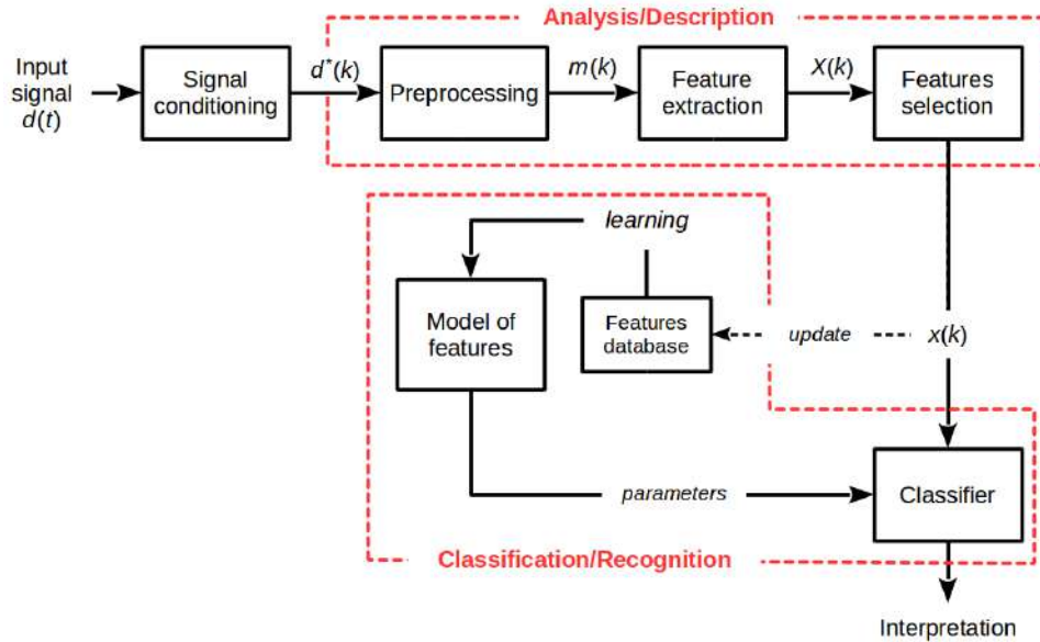
Figure 6: Block diagram of a general pattern recognition system.
