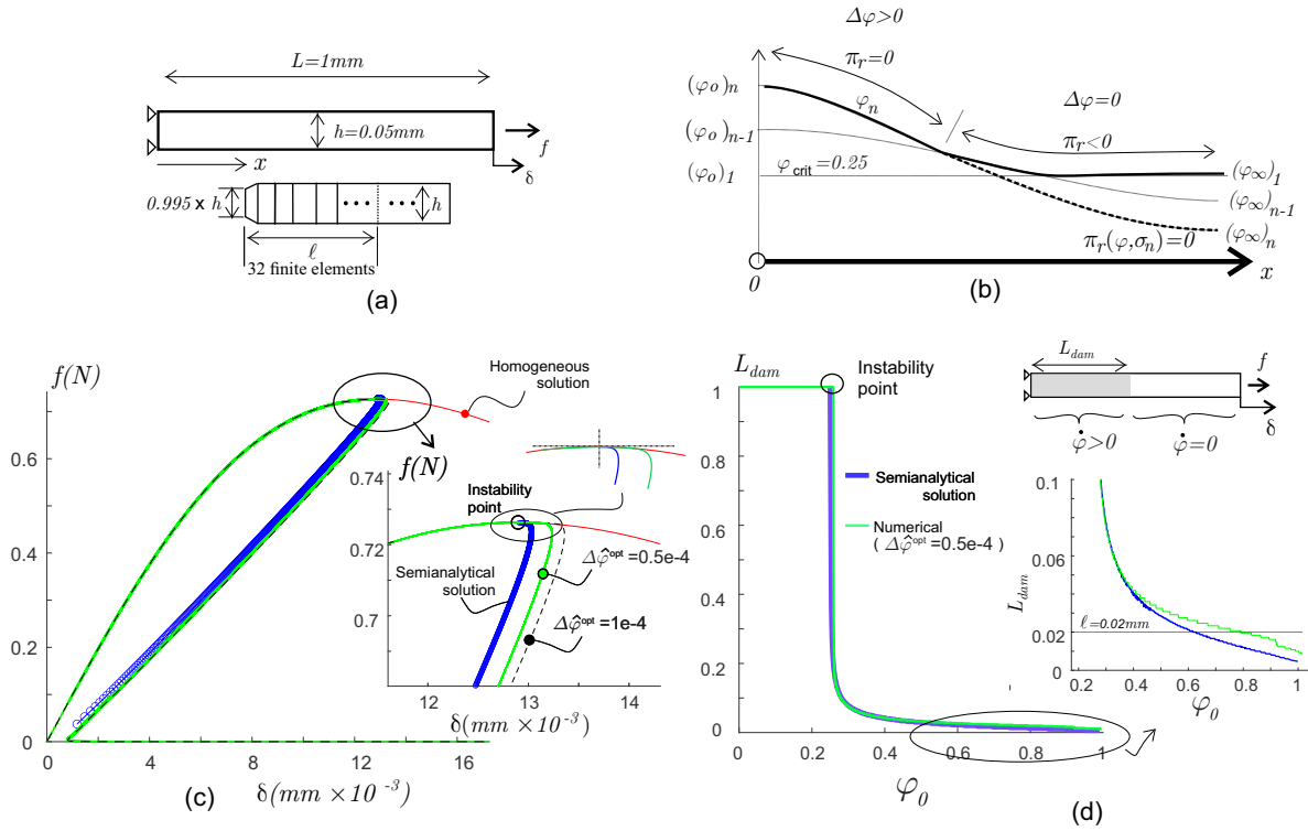
Figura D.1: Bar under tensile load. a) Geometrical perturbation and material properties. b) Semi-analytical procedure satisfying the complementarity conditions. c) Force versus displacement plot. Curves corresponding to the homogeneous and localized solutions have horizontal tangent lines at the limit point. See further details in the inset. d) Size of the localization zone, L_{\text{dam}} , in terms of the maximum damage, \varphi_0 , in successive load steps.
