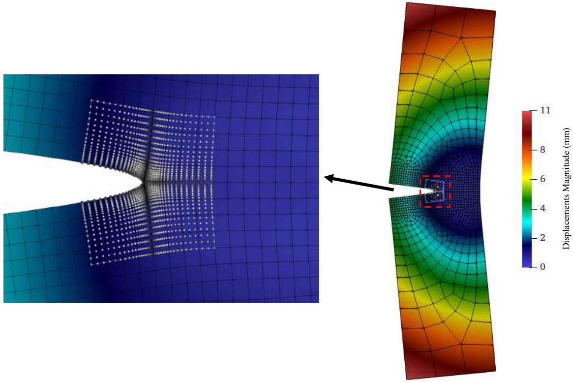
Figura F.15: Displacement magnitude using the proposed Ov-IEFG-FEM method for a SENT specimen.
