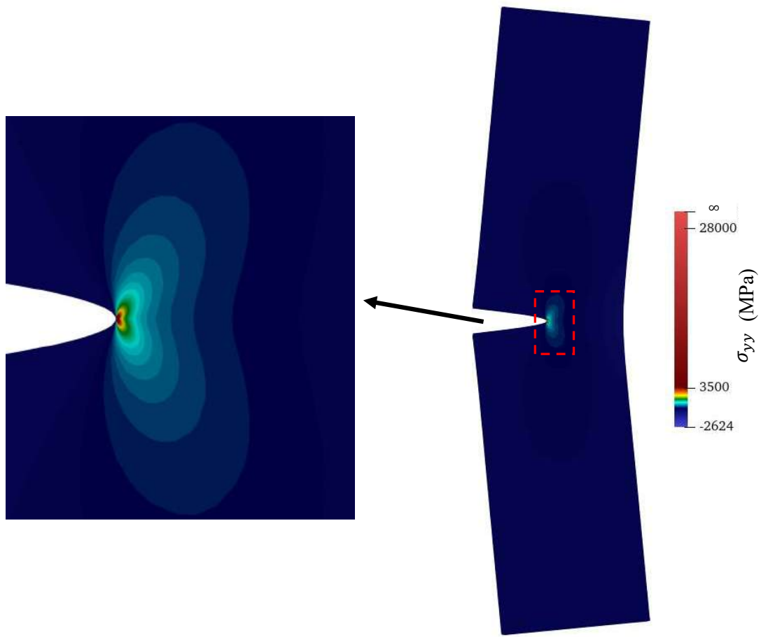
Figura F.16: \sigma_{yy} stress distribution using the proposed Ov-IEFG-FEM method for a SENT specimen in its deformed condition.
