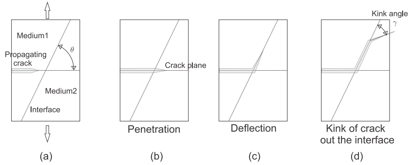
Figura A.4: Interaction modes between a propagating crack impinging on an interface at an angle \theta . a) Sketch of the problem. b) Penetration. c) Deflection. d) Kink of the crack out the interface, the crack leaving the interface form an angle \gamma .
