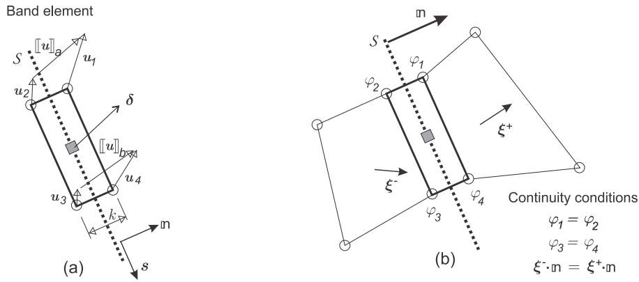
Figura A.15: Sketch of the technique used to implement jump conditions on the interface S . a) The band element is a slender finite element (quadrilateral in this case) on S featured with a regularized 3-D continuum damage model. b) Phase-field continuity conditions across the band element.
