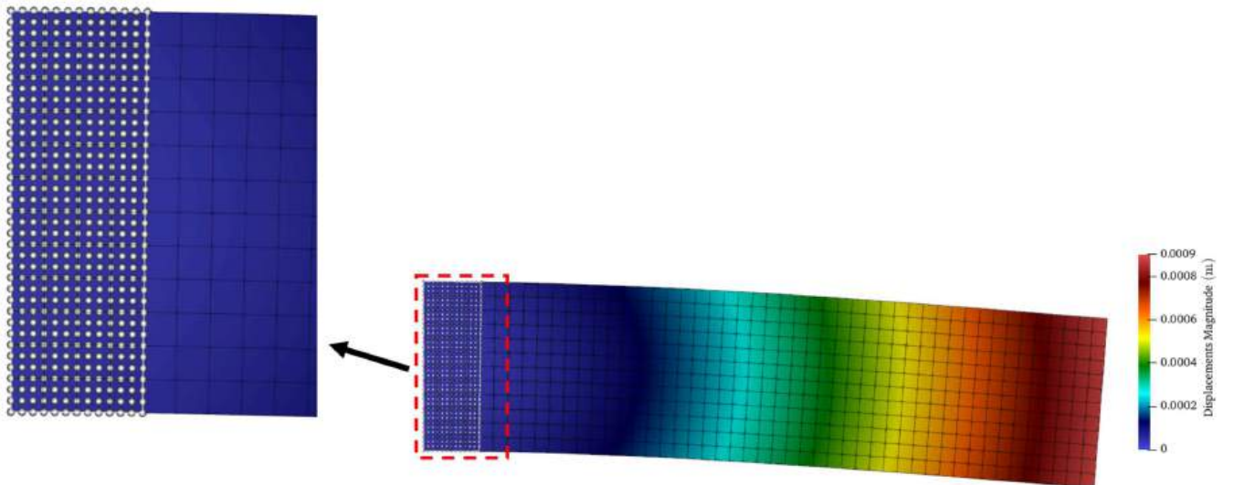
Figura F.4: Displacement magnitude by the proposed Ov-IEFG-FEM method for the cantilever beam.
