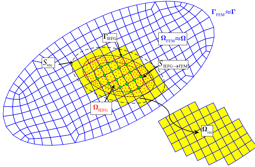
Figura E.1: Representation of the problem domain for a numerical solution performed via the proposed Ov-IEFG-FEM.
