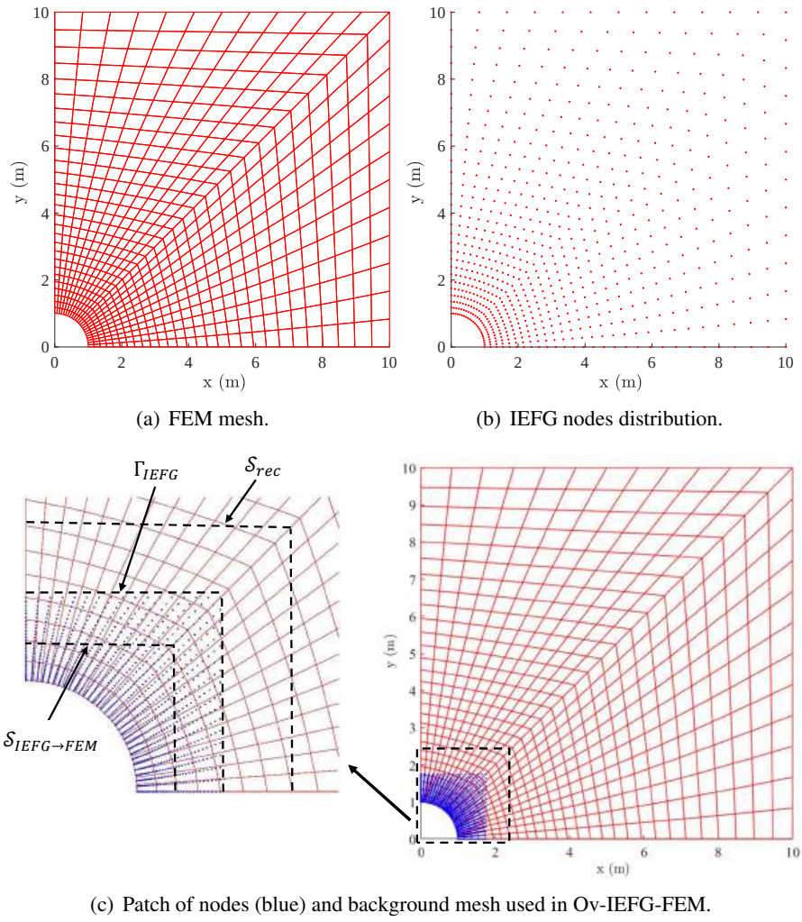
Figura F.8: Intermediate meshes and node distributions used in the convergence analysis for an infinite plate with a hole in the center.
