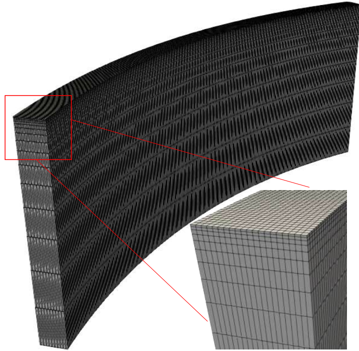
Figura E.24: Mesh used in the standard FEM-based solution of the 3-D problem of smaller dimensions, to be performed for numerical validation of the Ov-IEFG-FEM.
