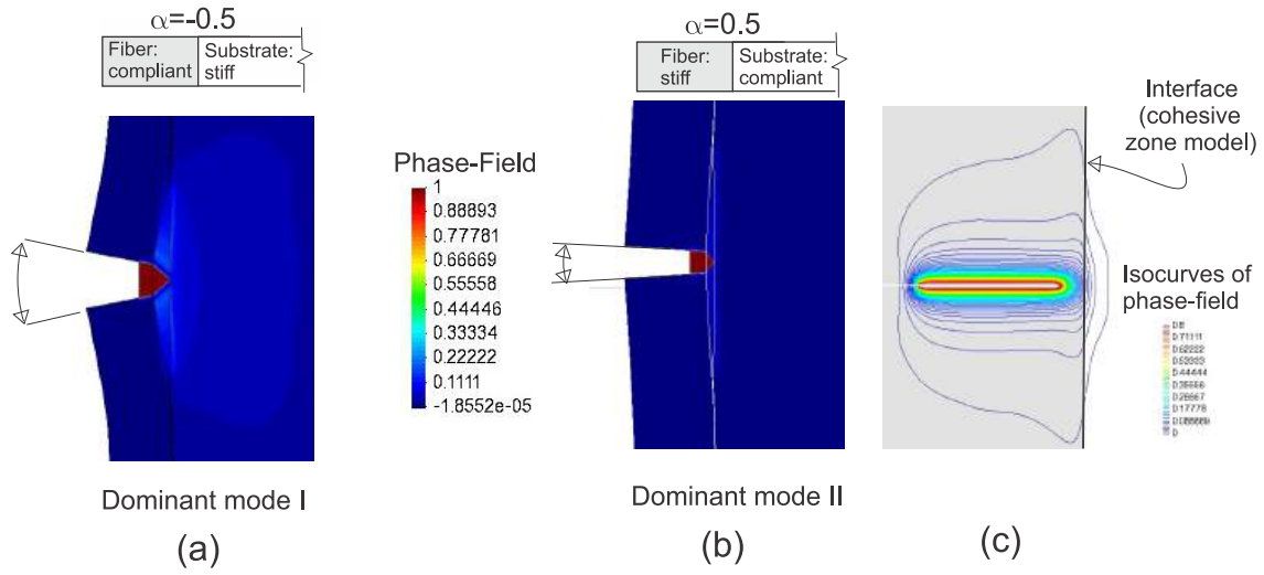
Figura A.8: Interaction analysis between a crack impinging an orthogonal interface with dissimilar fiber-substrate stiffness. a) Deformation mode of crack deviating into the interface: \alpha = -0.5 . The interface opening displays a dominant mode I. b) Deformation mode of crack deviating into the interface: \alpha = 0.5 . The interface opening displays a dominant mode II. c) Iso-curves of phase-field when the crack in the fiber is close to impinging the interface.
