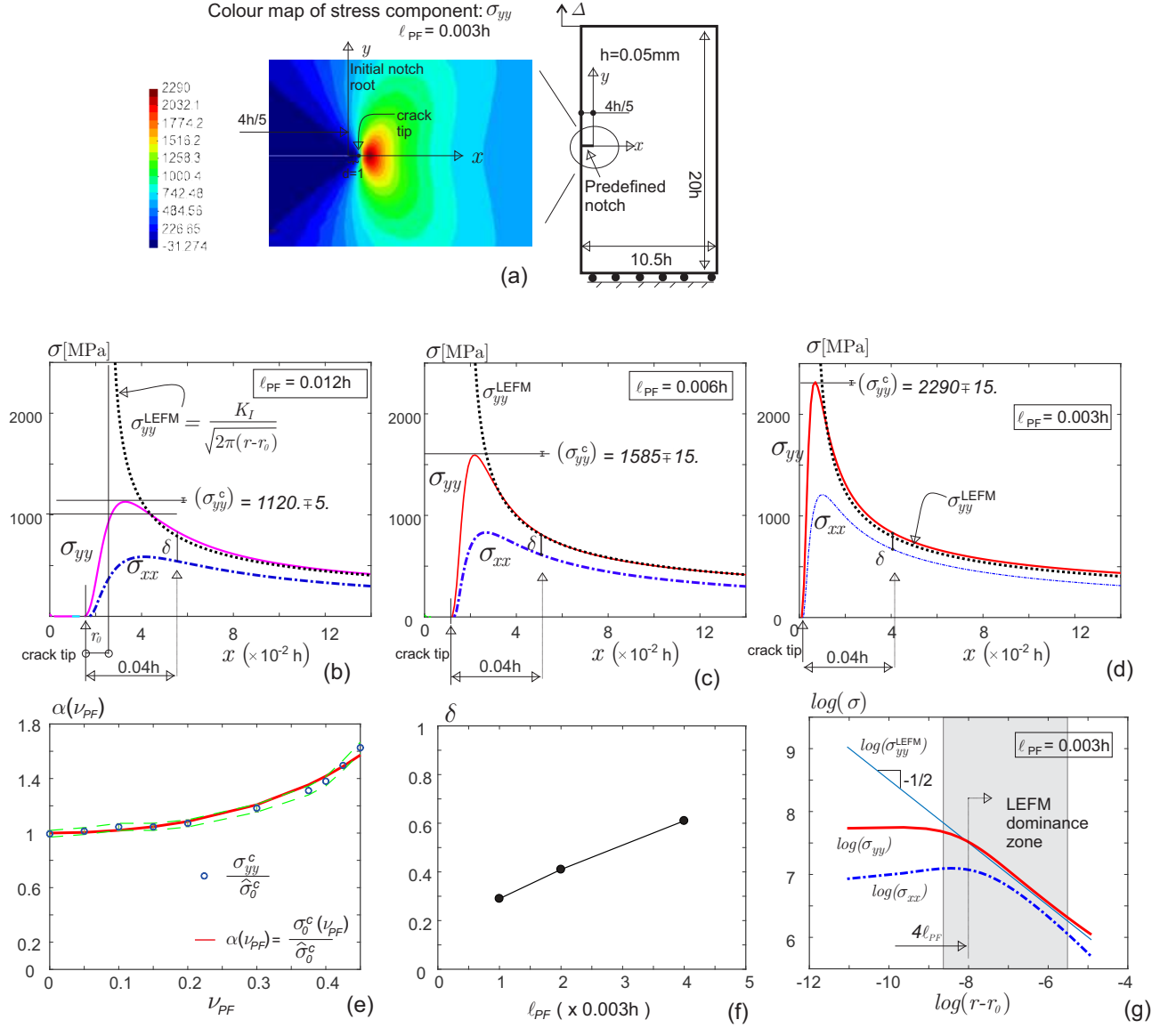
Figure A.3: Single Edge Notch Tension (SENT) specimen. Stress analysis near the crack-tip. a) specimen geometry and loading conditions. Stresses \sigma_{xx} , \sigma_{yy} and \sigma_{yy}^{LEFM} in the crack plane, along the x -axis: b) \ell_{PF} = 0.012h , c) \ell_{PF} = 0.006h , and d) \ell_{PF} = 0.003h . e) Peak stress coefficient, \alpha(\nu_{PF}) , as a function of the Poisson's ratio. f) Relative difference between stress components \sigma_{yy} and \sigma_{xx} , \delta = 2(\sigma_{yy}(x) - \sigma_{xx}(x))/(\sigma_{yy}(x) + \sigma_{xx}(x)) , evaluated at a distance x - r_0 = 0.04h of the estimated crack tip. g) Plot log-log of stresses \sigma_{xx} , \sigma_{yy} and \sigma_{yy}^{LEFM} in the crack plane, along the x -axis with \ell_{PF} = 0.003h .
