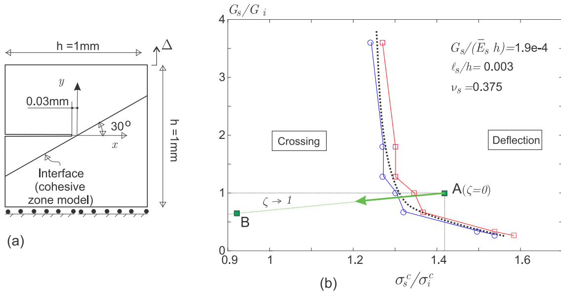
Figura A.9: Interaction between a propagating crack impinging an inclined interface. a) Specimen geometrical configuration. b) The limit curve in black dotted line separates the regions where deflection, or crossing, are observed. Points in red square represent solutions displaying a propagating crack deflecting into the inclined interface. Points in blue circles represent cracks crossing the interface.
