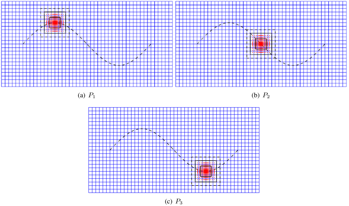
Figura E.12: Patch nodes (red) and background mesh used to solve the transient heat conduction problem over the rectangular thin plate with the moving heat source following a sinusoidal scanning path.
