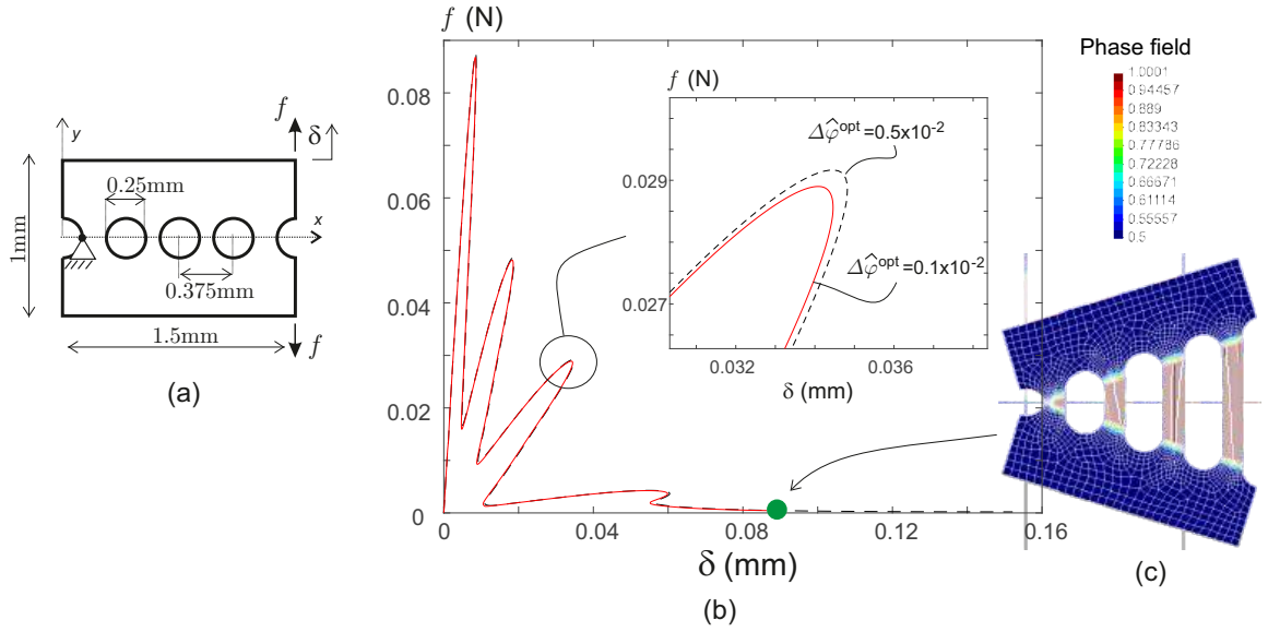
Figura D.9: Perforated plate. a) Specimen geometry. b) Force f versus displacement \delta curves.
