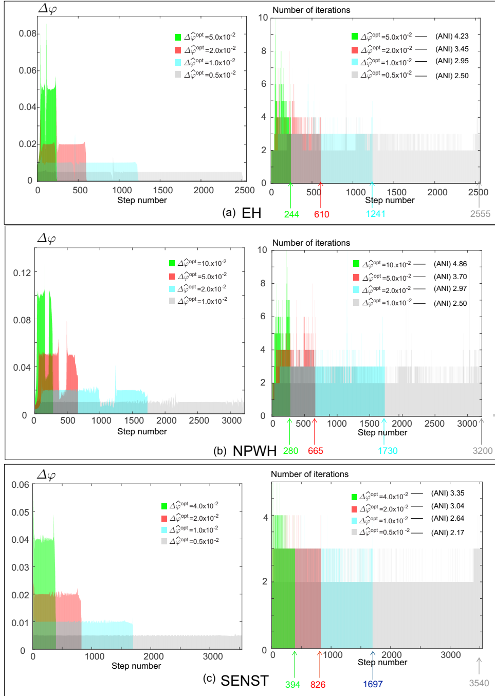
Figura D.10: Performance analysis. a) EH. b) NPWH, and c) SENST test. Left column: phase field increase ( \Delta\varphi = \|(\varphi_n - \varphi_{n-1})\|_\infty ) in each staggered scheme step (Step Number). Right column: number of iterations required by the mechanical stage solution in each staggered scheme step. Load versus displacement plots for the here reported tests, EH, NPWH, and SENST, are shown in Figures D.8-b, D.5-c, and D.6-b, respectively.
