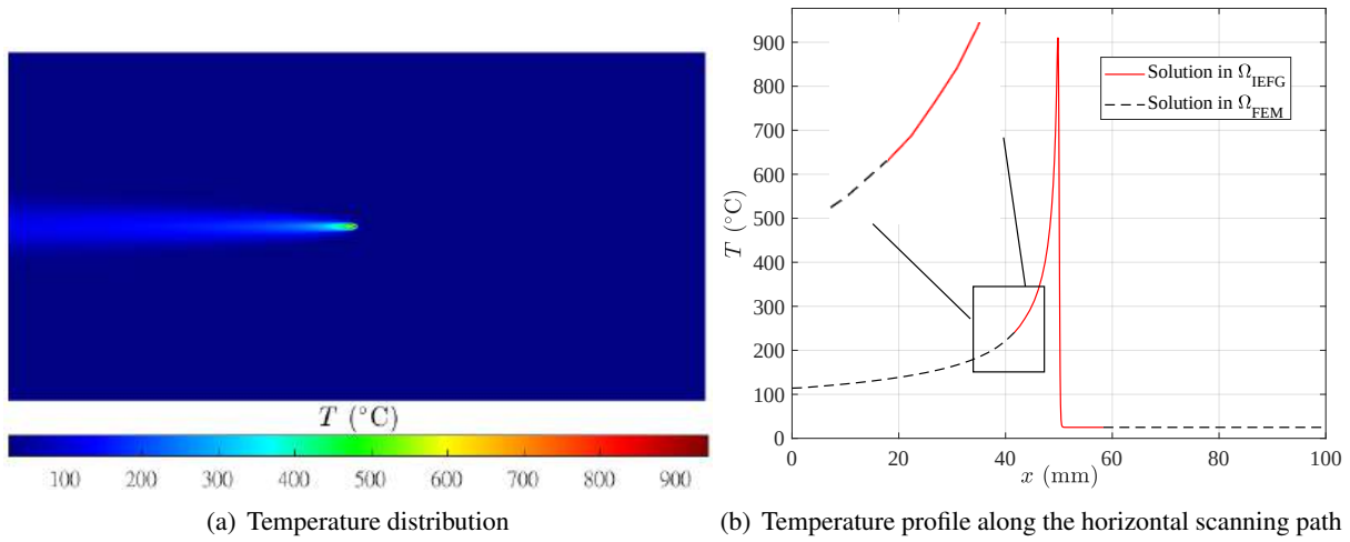
Figura E.29: Stable results obtained via the Ov-IEFG-FEM with advection dominating the heat transfer problem in the moving domain \Omega_{IEFG} , when it is solved under the SUPG stabilised formulation.
