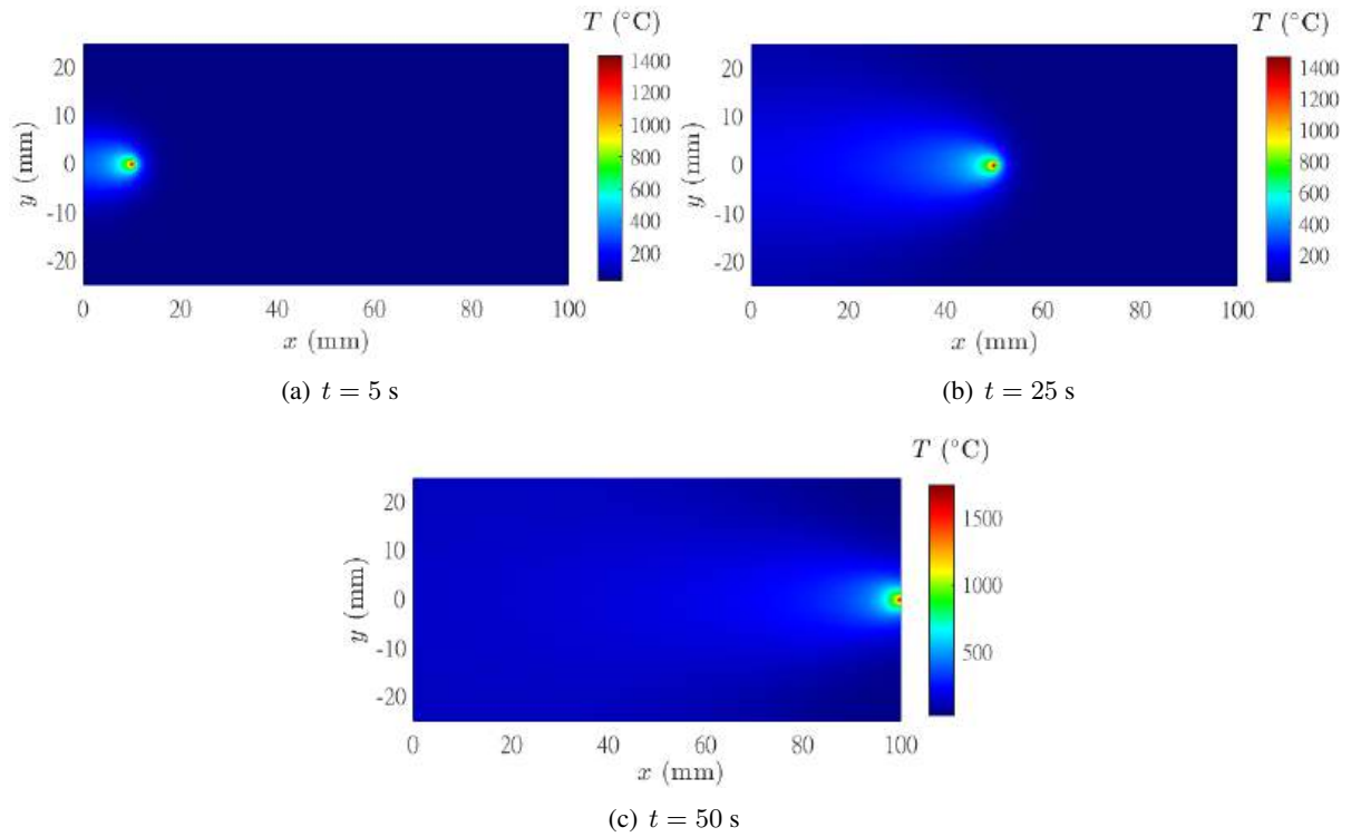
Figure E.8: Temperature distributions computed via the proposed Ov-IEFG-FEM, with the patch nodes actually following the horizontal scanning path of the moving heat source.
