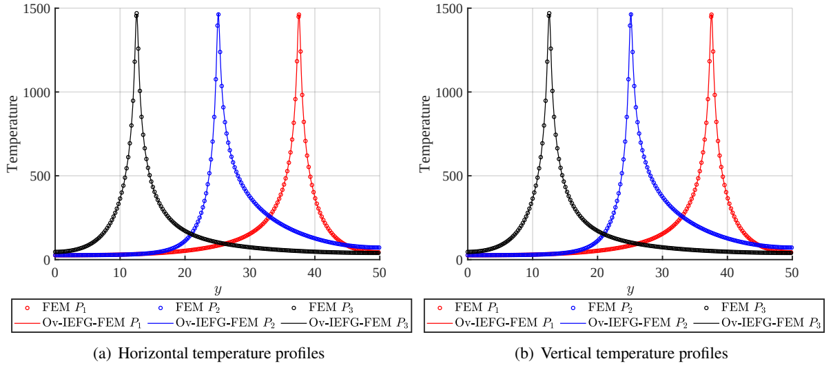
Figura E.15: Temperature profiles computed along the horizontal and vertical axes passing over the current heat source position, comparison between the results computed via the proposed Ov-IEFG-FEM and a very fine FEM-based solution.
