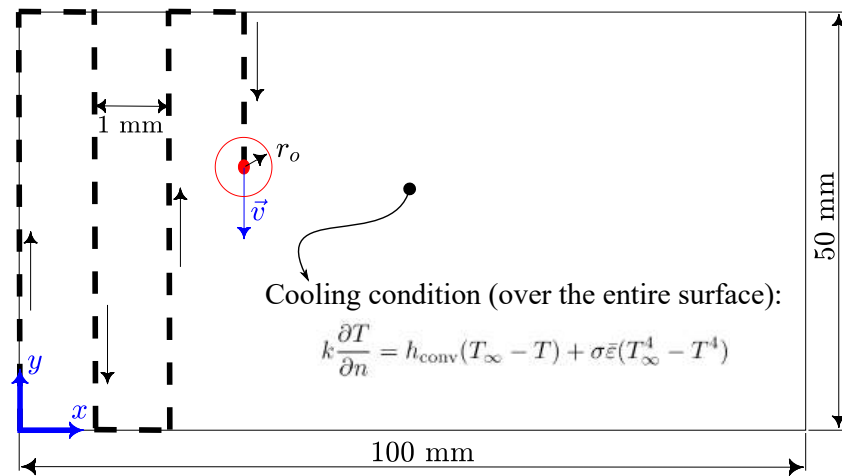
Figura E.16: Representation of the transient heat conduction problem over the rectangular thin plate with a moving heat source following a S-type path.
