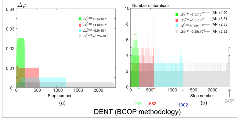
Figura D.11: Performance analysis. DENT test using the Bound-Constrained Optimization Problem (BCOP) methodology for solving the micro-force balance equation. Left column: phase field increase ( \Delta\varphi = \|(\varphi_n - \varphi_{n-1})\|_\infty ) in each staggered scheme step (Step Number). Right column: number of iterations required by the mechanical stage solution in each staggered scheme step.
