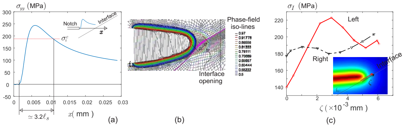
Figura A.14: Shield effect induced by the interface degradation. a) Stress field \sigma_{yy}(x) ahead of the crack tip, along the x -axis. b) Deformed mesh displaying the interface opening before the crack impinges on the interface. c) Principal stress, \sigma_I , along lines parallel to the interface, on the left and right points of the substrate.
