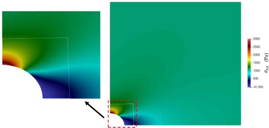
Figura F.10: Distribution of the \sigma_{xx} stress component achieved via the proposed Ov-IEFG-FEM for the infinite plate with a centered hole benchmark problem.
