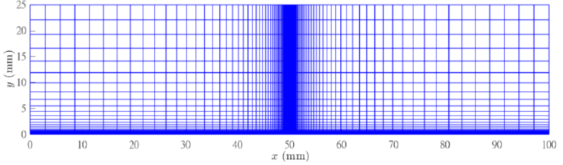
(a) FEM, 172 \times 43 = 7,396 elements (7,612 nodes)
