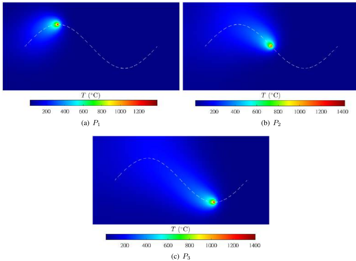
Figura E.13: Temperature distributions computed via the proposed Ov-IEFG-FEM, with the patch nodes following the sinusoidal scanning path of the moving heat source.
