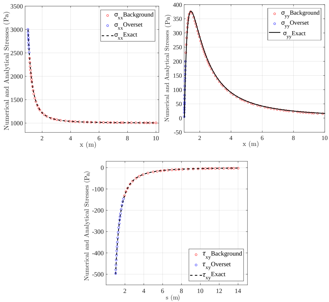
Figura F.11: \sigma_{xx} and \sigma_{yy} stress components computed via the Ov-IEFG-FEM along the horizontal line (x, 0) , and \tau_{xy} stress component computed along the arc length s of a diagonal 45^\circ line. For comparison, the numerical results have been plotted over the analytical solution.
