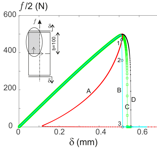
Figura D.12: Double-edged notched test (DENT). Solutions obtained with: arc-length procedure (curve A); variant I and \Delta\delta/b = 25. \times 10^{-6} (curve B); variant II and \Delta\delta/b = 2.5 \times 10^{-6} (curve C); variant II and \Delta\delta/b = 5. \times 10^{-6} (curve D).
