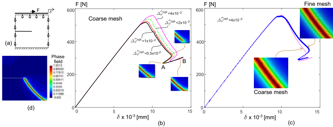
Figura D.6: Single edge notched shear test (SENST). a) Specimen geometry and boundary conditions. b) Coarse mesh: total shear force F on the top boundary versus displacement \delta . The insets show the phase field variable evolution in three instants as the snap-back develops along the equilibrium curve. Phase field tip enrichment (PFTE) has been assumed. c) F versus \delta curves, coarse and fine meshes with \Delta\hat{\varphi}^{opt} = 4 \times 10^{-2} . Points of the fine mesh result indicate load steps. d) Crack path at the end of the analysis ( \delta = 0.014\text{mm} ).
