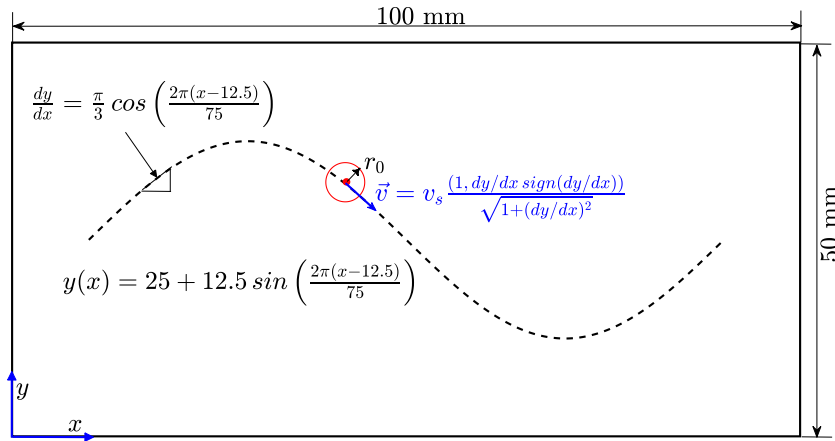
Figura E.11: Representation of the transient heat conduction problem over the rectangular thin plate with a moving heat source following a sinusoidal scanning path.
