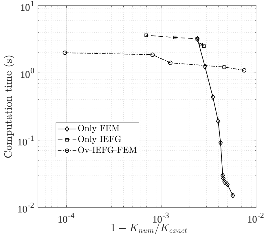
Figura F.21: Comparison of CPU times as a function of K_I normalization for each of the implemented techniques.
