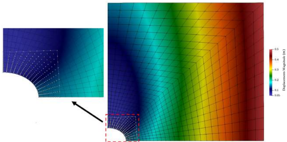
Figura F.9: Displacement magnitude using the proposed Ov-IIEFG-FEM method for an infinite plate with a hole at the center in its deformed condition.
