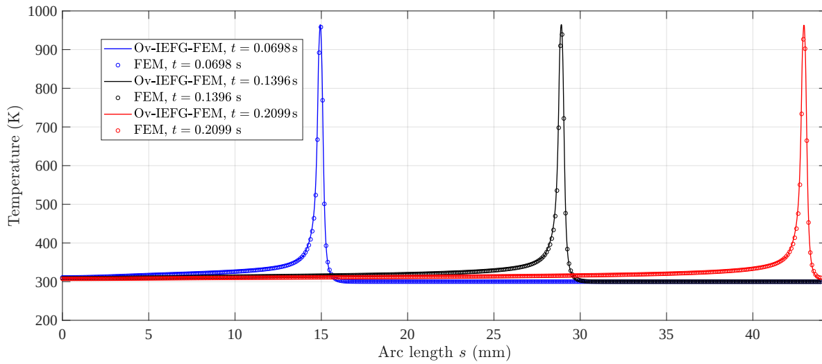
Figura E.25: Comparison of the temperature profile computed via the Ov-IEFG-FEM along the arc length s covered by the moving heat source, with those obtained from a standard FEM-based solution.
