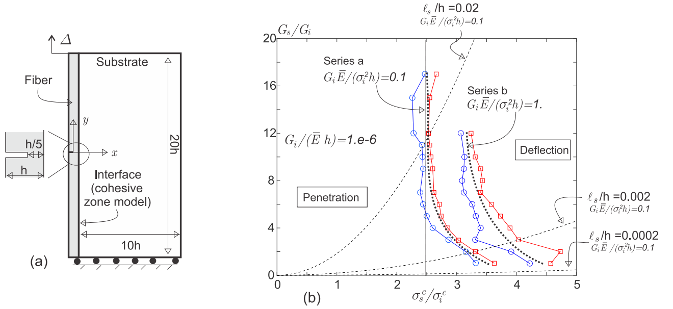
Figure A.6: Interaction analysis among a crack impinging an orthogonal interface with similar fiber-substrate stiffness. a) Geometrical configuration of the laminated edge-cracked panel. b) Analysis with identical fiber and substrate properties (Dundurs's parameters are \alpha = \beta = 0 ). Series a and b of tests are shown. Points in red squares represent solutions displaying a propagating crack deflecting into the interface. Points in blue circles represent solutions displaying a propagating crack penetrating the substrate.
