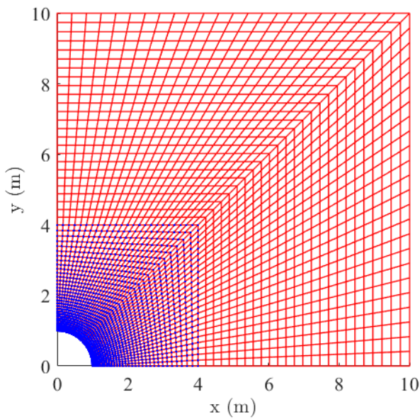
(b) Ov-IEFG-FEM fitted
