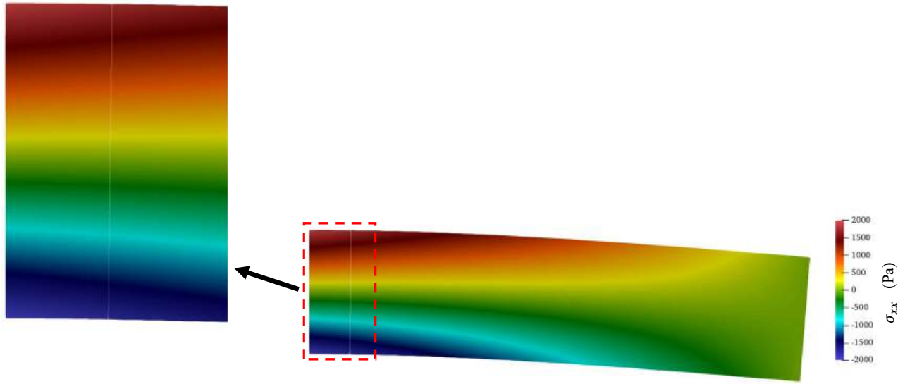
Figura F.5: Stress distribution \sigma_{xx} by the proposed Ov-IEFG-FEM method for the cantilever beam in its deformed condition.
