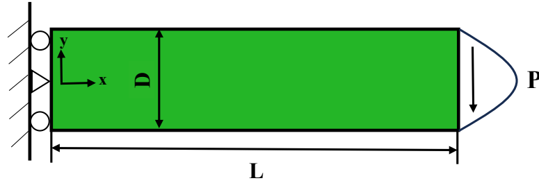
Figura F.2: Representation of geometry and boundary conditions for a cantilever beam.
