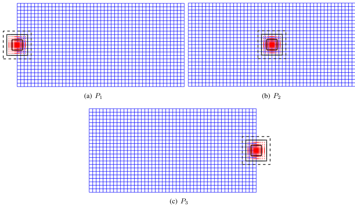
Figura E.17: Patch nodes (red) and background mesh used to solve the transient heat conduction problem over the rectangular thin plate with the moving heat source following a S-type scanning path.
