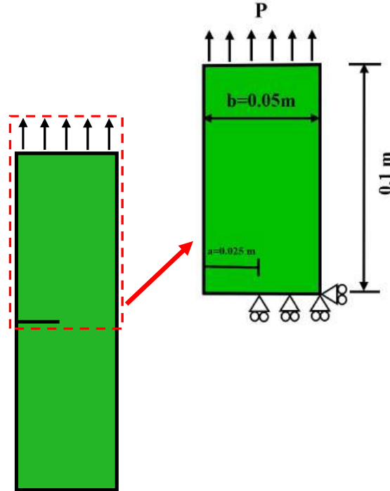
Figura F.13: Representation of geometry and boundary conditions for a Single Edge Notched Tension (SENT) specimen.
