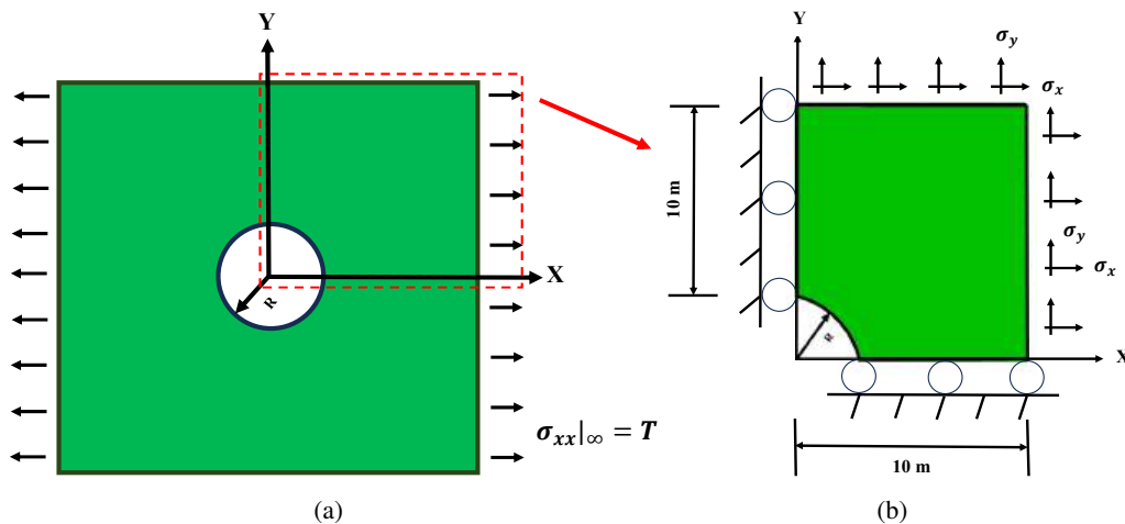
Figura F.7: Representation of geometry and boundary conditions for an infinite plate with a centered hole.
