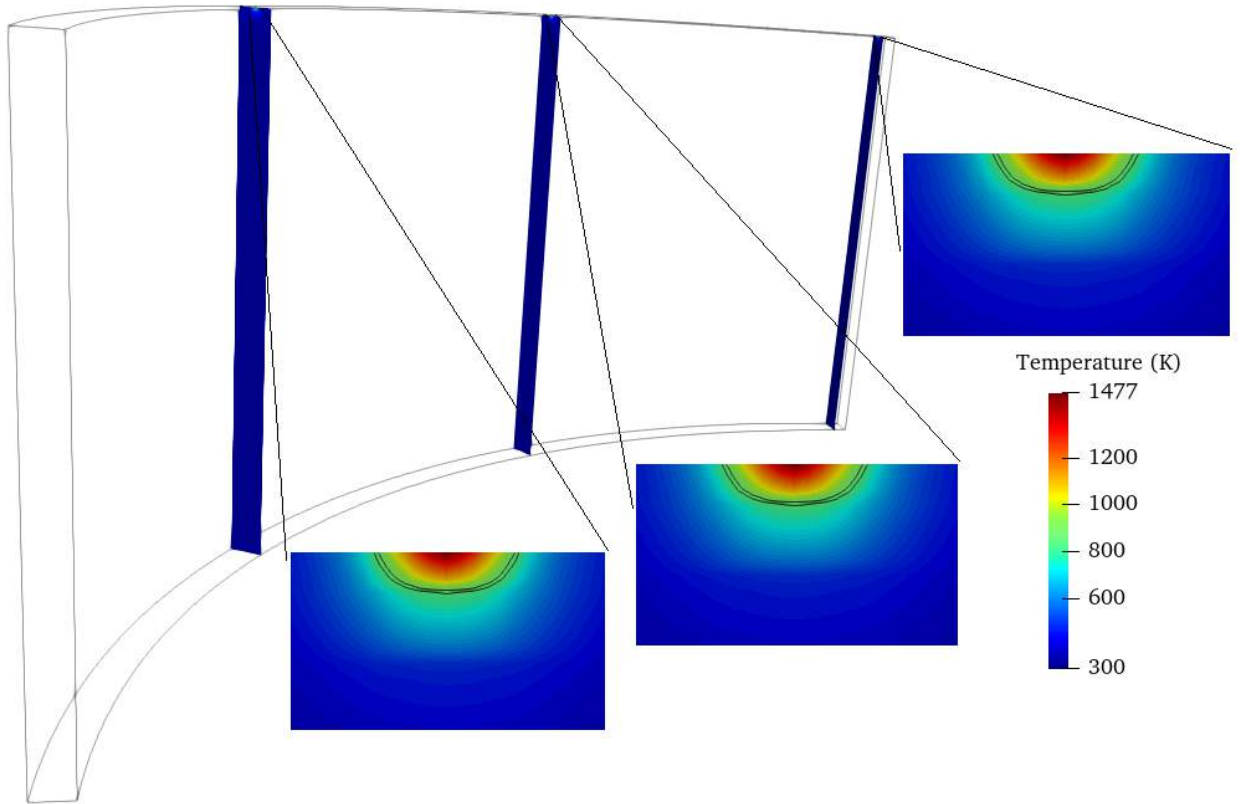
Figura E.22: Temperature distributions in axial slices located at the position occupied by the moving heat source at different times.
