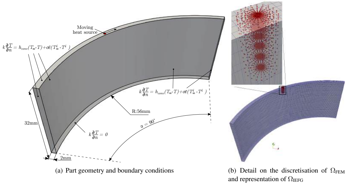
Figura E.20: Configuration and boundary conditions of the three-dimensional problem with curved geometry and temperature-dependent material properties, and detail of the arc-shaped part discretisation via FEM and representation of the region near the moving heat source with the overlapping patch nodes for IIEFG computations.
