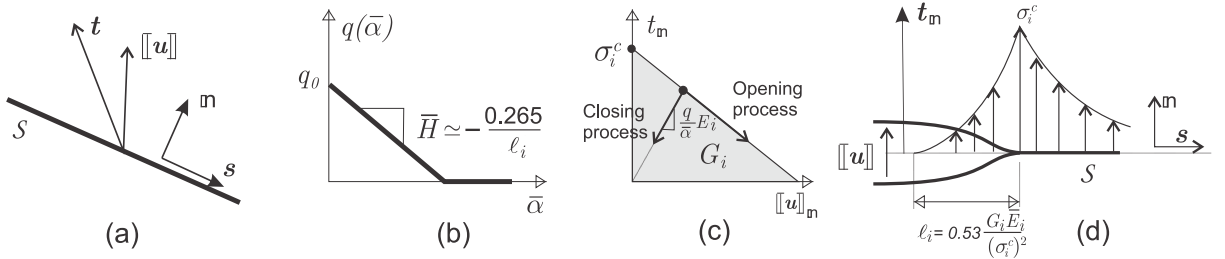
Figura A.2: Interface cohesive model. a) traction \mathbf{t} and separation [\![\mathbf{u}]\!] vectors at the interface. b) Softening law, q(\bar{\alpha}) , governing the traction-separation degradation. c) Traction-separation law of an interface opening in mode I. The area below the curve is equal to the fracture energy G_i and the peak stress component is \sigma_i^c . d) Estimation of the cohesive characteristic length \ell_i .
