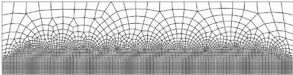
Figure E.9: Mesh refined along the scanning path for the FEM-based solution of the transient heat conduction problem over the rectangular thin plate with a moving heat source following a horizontal straight path.
