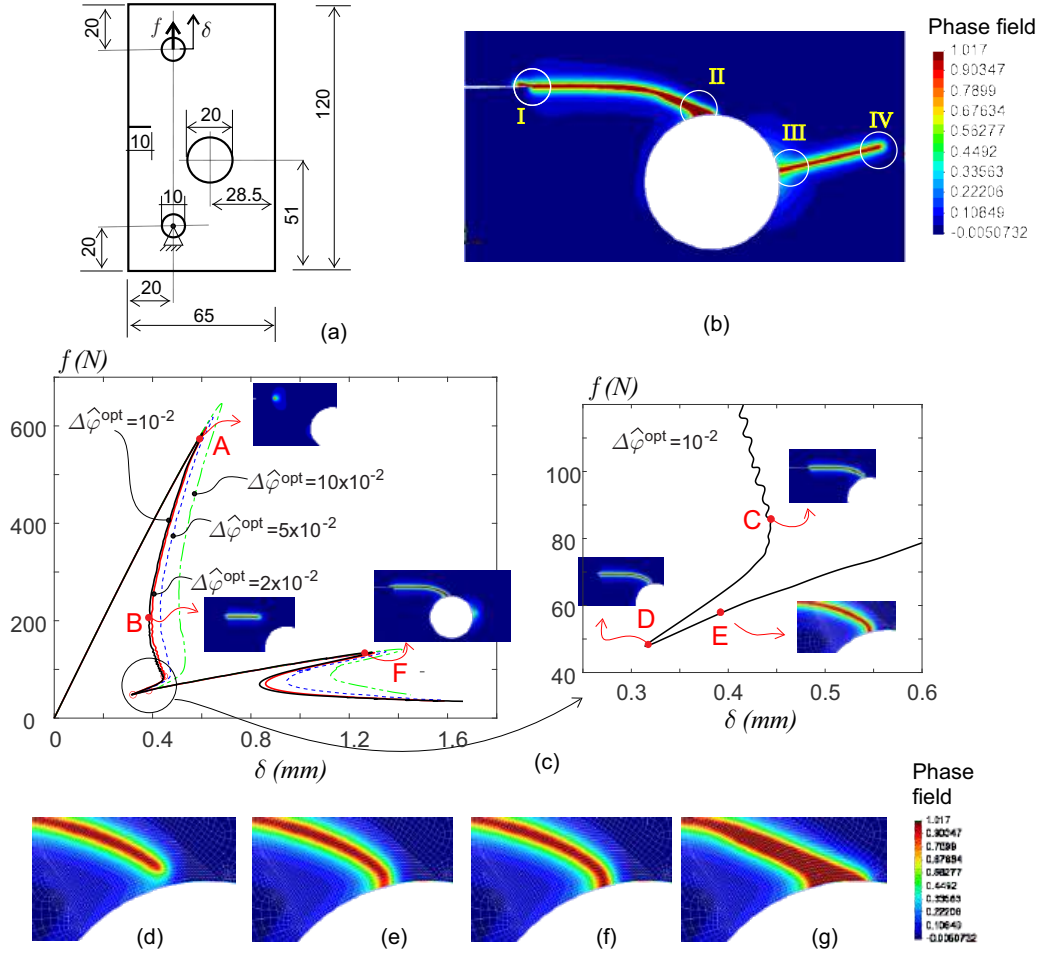
Figura D.5: Notched plate with a hole (NPWH). a) Specimen geometry. b) Crack path at the end of the analysis ( \delta = 2mm ). c) Force f versus displacement \delta . d), e), f), and g) Sequence of crack advance images when the crack intersects the hole. Images: d), e), f), and g) correspond to Points C, D, E, and F in the equilibrium curve, respectively.
