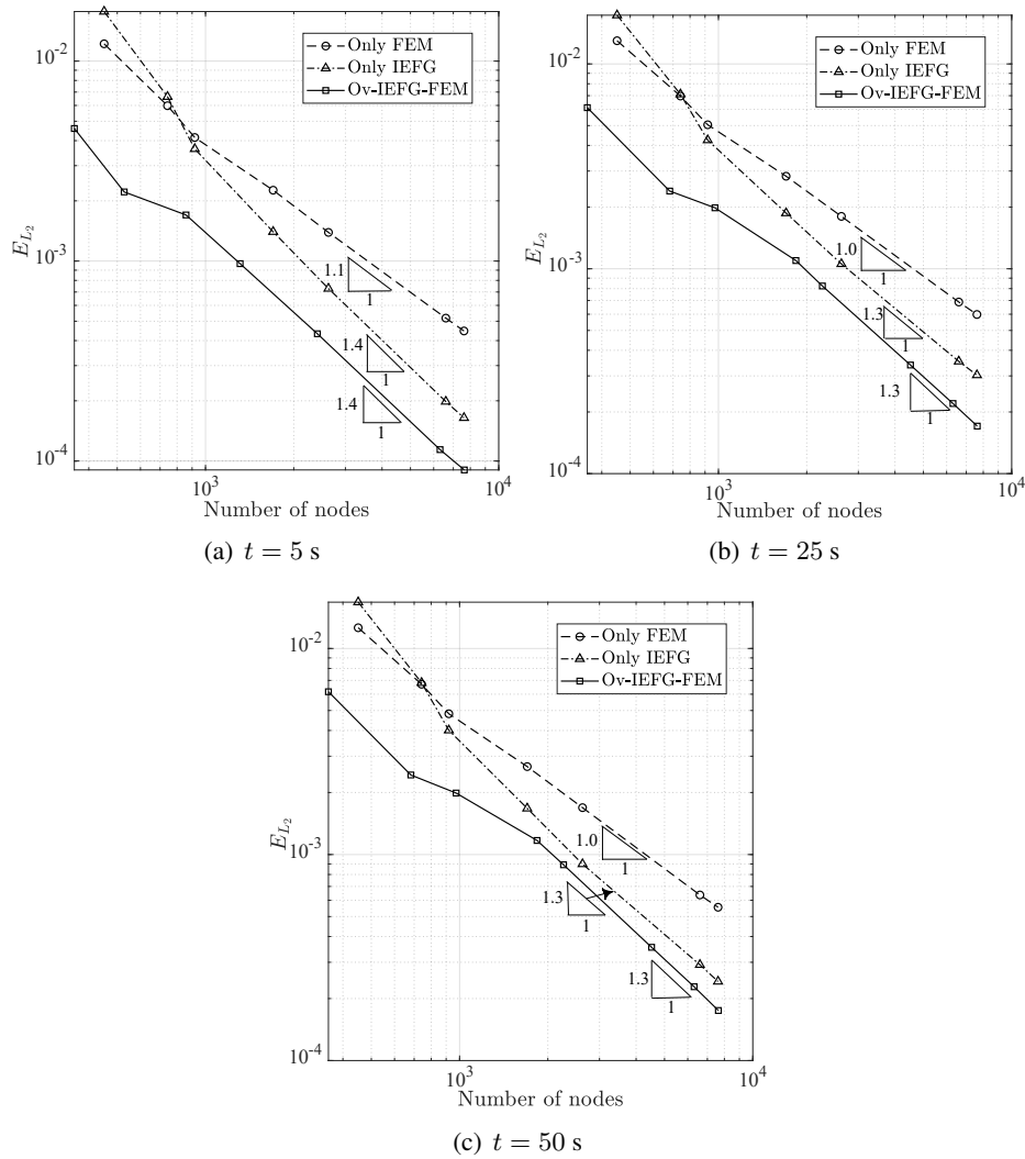
Figura E.5: Convergence behaviour of FEM, IEFG, and the proposed Ov-IEFG-FEM at different times.
