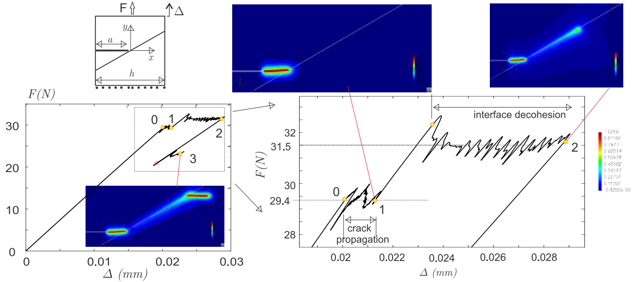
Figura A.12: Analysis of a crack kinking out of an interface. Structural load F versus displacement \Delta curve (left plot) and detail of the peak loads (right plot). Mesh with h^e = 7.5 \times 10^{-4} \text{ mm} . Point 0 identifies the initiation of crack propagation; Point 1 identifies the crack impinging on the interface; Point 2 identifies the crack abandoning the interface; Point 3 corresponds to the end of analysis.
