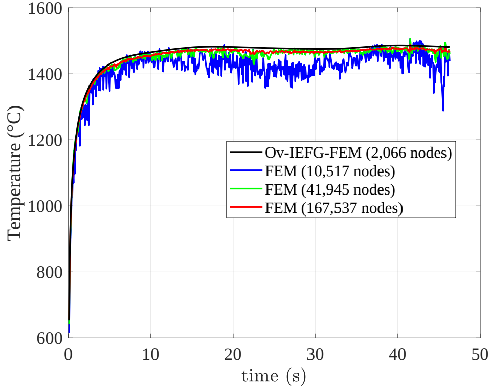
Figura E.26: Temperature at the position occupied by the moving heat source at different times for the 2-D benchmark problem of the moving heat source following a sinusoidal path.
