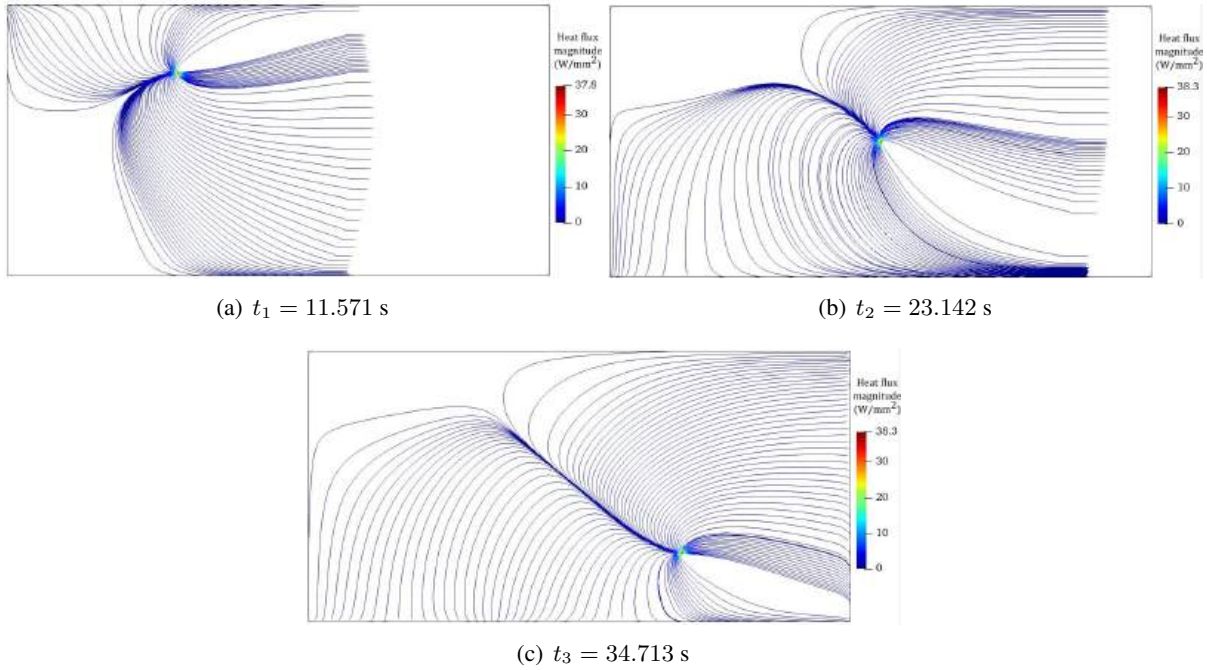
Figura E.27: Heatlines achieved via the computation of a continuous heat flux field under the proposed Ov-IEFG-FEM.
