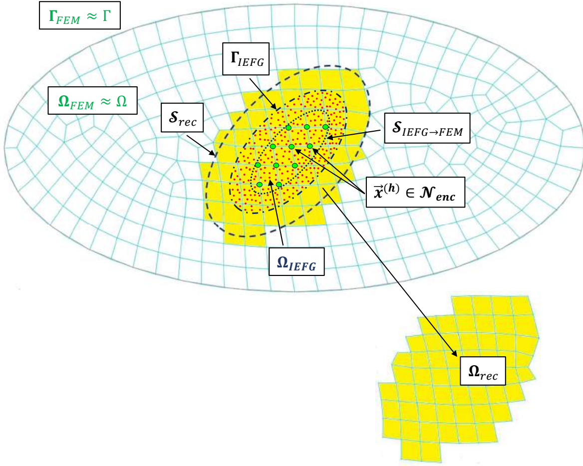
Figura F.1: Representation of the problem domain for a numerical solution performed via the proposed Ov-IEFG-FEM
