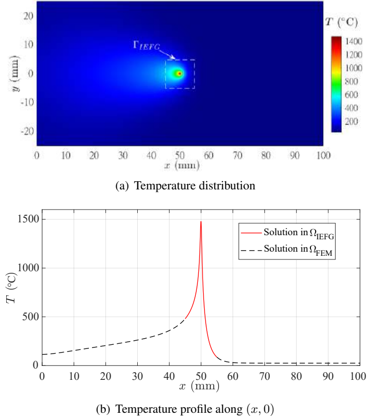
Figura E.6: Solution obtained via the Ov-IEFG-FEM at t = 25 s under Rosenthal's coordinates transformation. Although the numerical solution has been performed at the upper half of the plate, the corresponding temperature distribution is plotted in (a) over the entire plate for better visualisation.
