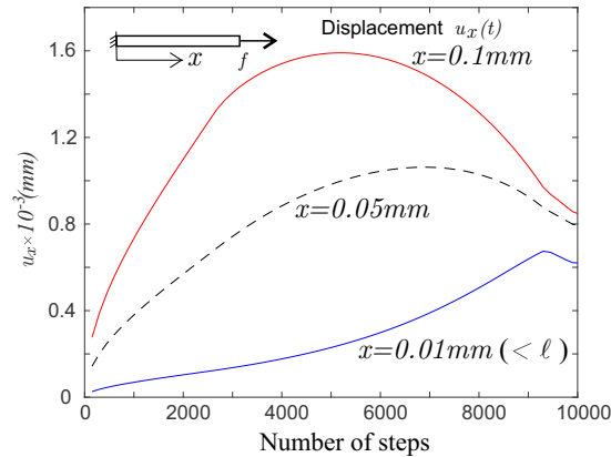
Figura D.2: Bar under tensile load. Displacements, u_x , of bar points at coordinates: x = 0.1\text{mm} , x = 0.05\text{mm} , and x = 0.01\text{mm} versus number of load step. Solution with \Delta\hat{\varphi}^{\text{opt}} = 0.5 \times 10^{-4} .
