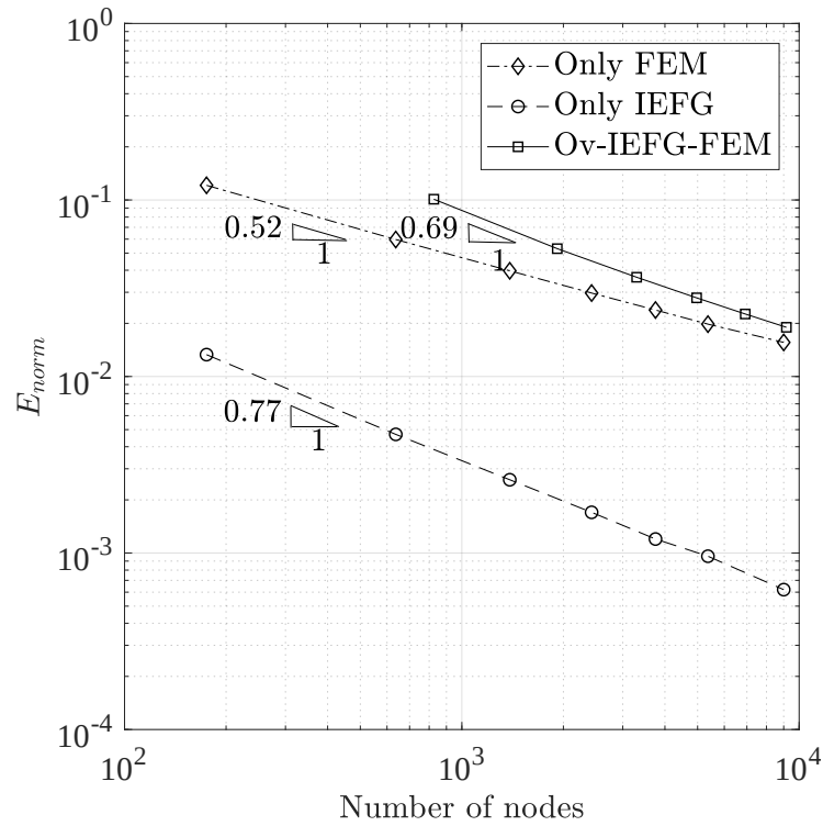
Figura F.6: Convergence behavior of FEM, IEFG, and the proposed Ov-IEFG-FEM for the cantilever beam.
