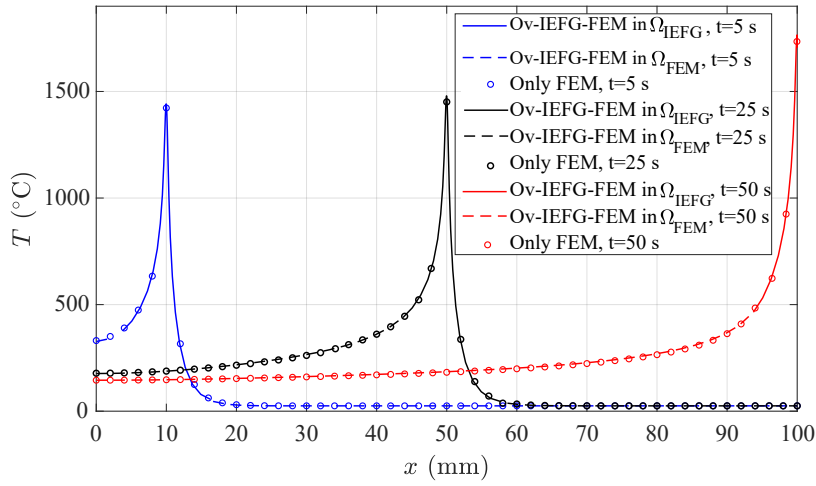
Figura E.10: Temperature profiles computed along the horizontal scanning path via the proposed Ov-IEFG-FEM with moving patch nodes, compared to the standard FEM-based solution.
