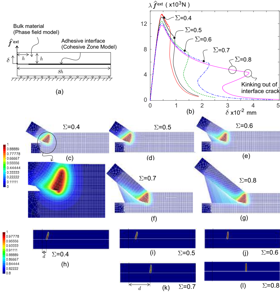
Figura D.7: Adhesively-bonded composite. a) Specimen geometry and load. b) Force \lambda \hat{f}^{ext} versus displacement \delta . c) d), e), f), and g) deformed meshes and phase field distribution at the end of the analysis. h), i), j), k), and l) crack path in the plate at the end of the analysis.
