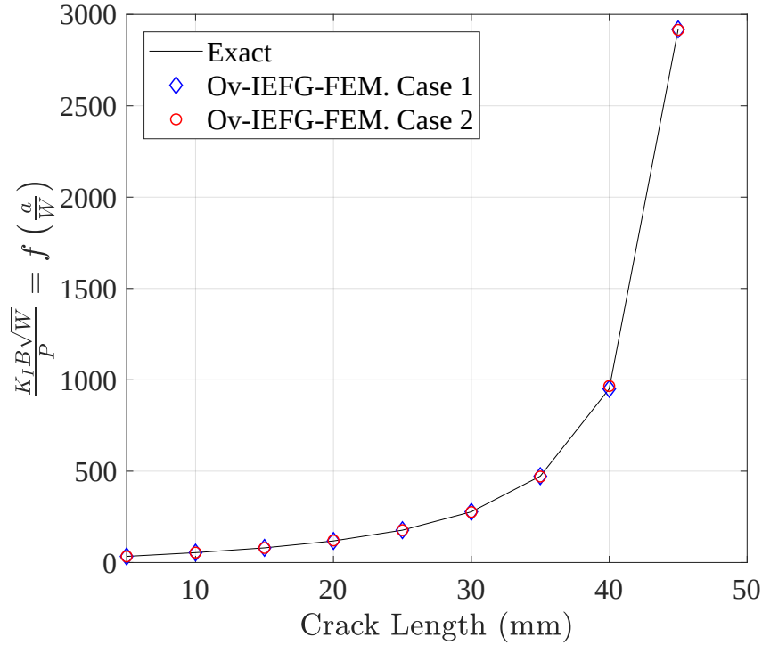
Figura F.20: Comparison of K_I values between reference solution [1] and the proposed Ov-IIEFG-FEM for case 1: Structured FEM background mesh and case 2: Distorted FEM background mesh.
