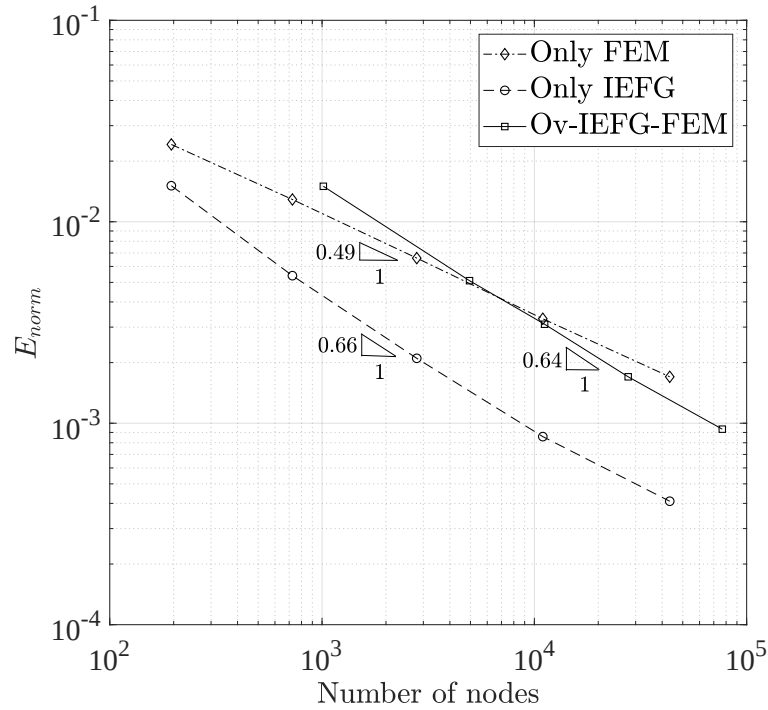
Figura F.12: Convergence behavior of FEM, IEFG, and the proposed Ov-IEFG-FEM for an infinite plate with a hole at the center.
