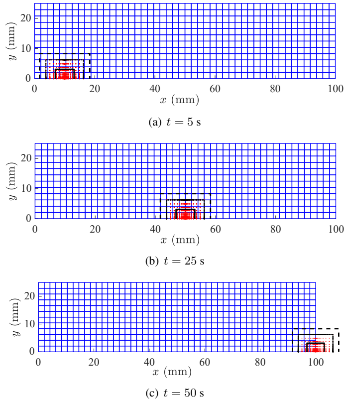
Figura E.7: Patch nodes (red) and background mesh used to solve the transient heat conduction problem over the rectangular thin plate, with the patch nodes actually following the simple horizontal scanning path of the moving heat source. The black dashed lines represent \mathcal{S}_{\text{rec}} . The temperature \bar{T}_{\text{FEM}} is imposed (integrated) on \Gamma_{\text{IEFG}} using the Gauss points located on it (black points), whereas \bar{T}_{\text{IEFG}} is reciprocally imposed at those nodes h of the background mesh that are enclosed by \mathcal{S}_{\text{IEFG} \rightarrow \text{FEM}} (black solid line).
