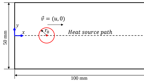
Figura E.2: Representation of the benchmark problem to be solved under the Rosenthal's formulation for accuracy and convergence analysis of the proposed Ov-IEFG-FEM.
