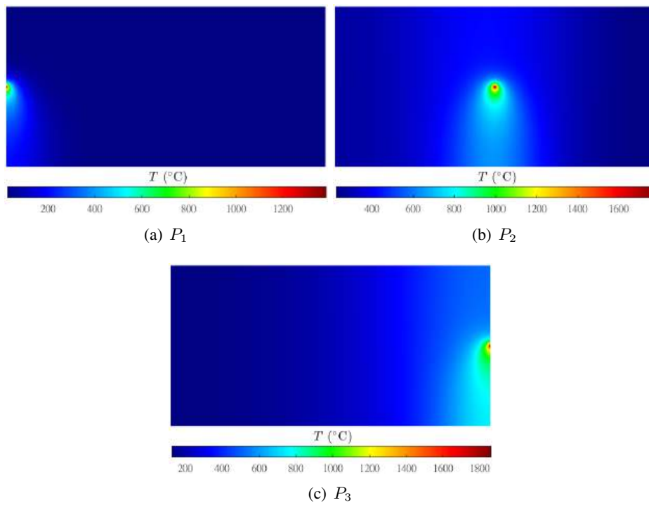
Figura E.18: Temperature distributions computed via the proposed Ov-IEFG-FEM, with the patch nodes following the S-type scanning path of the moving heat source.
