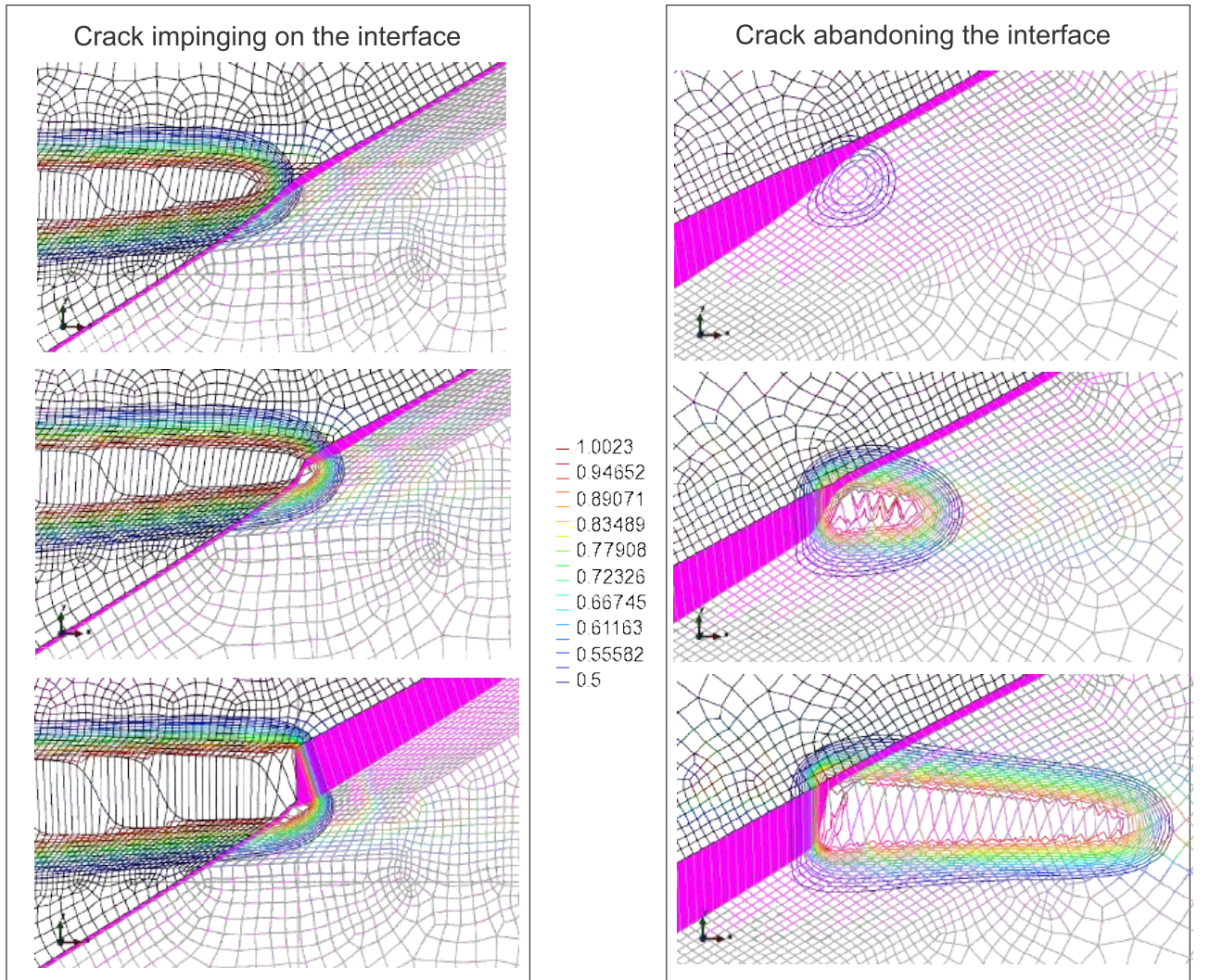
Figura A.11: Analysis of a crack kinking out of an interface. Sequence of deformed meshes and phase-field iso-curves, at different stages of the loading process. Mesh with h^e = 7.5 \times 10^{-4}mm . Left column: the crack impinges on the interface. Right column: the crack abandons the interface.
