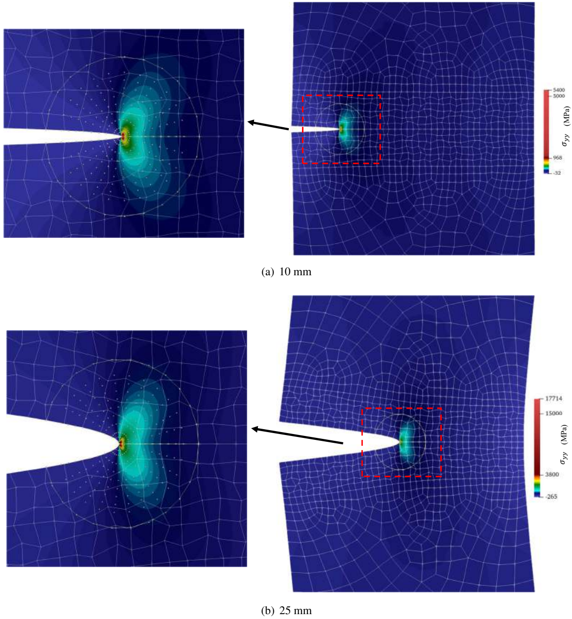
Figura F.19: \sigma_{yy} stress distribution for SENT specimen with distorted background mesh for different crack lengths.
