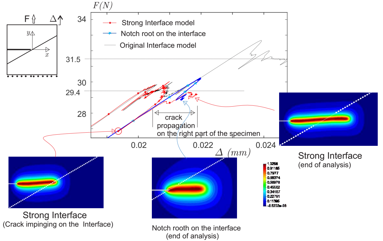
Figure A.13: Curves F vs. \Delta of three tests. a) Strong interface (red curve). b) Notch root intersecting the interface (blue curve). c) Original test taken from Figure A.12 (black curve).
