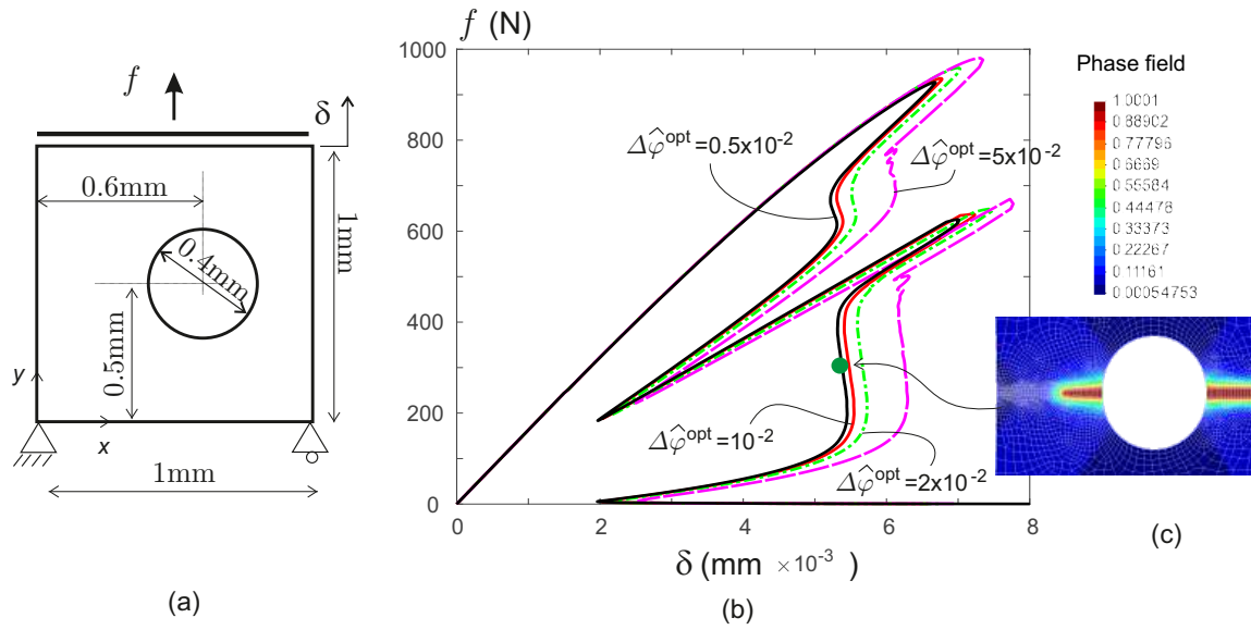
Figura D.8: Plate with an eccentric hole (EH). a) Specimen geometry. b) Total force f versus displacement \delta .
