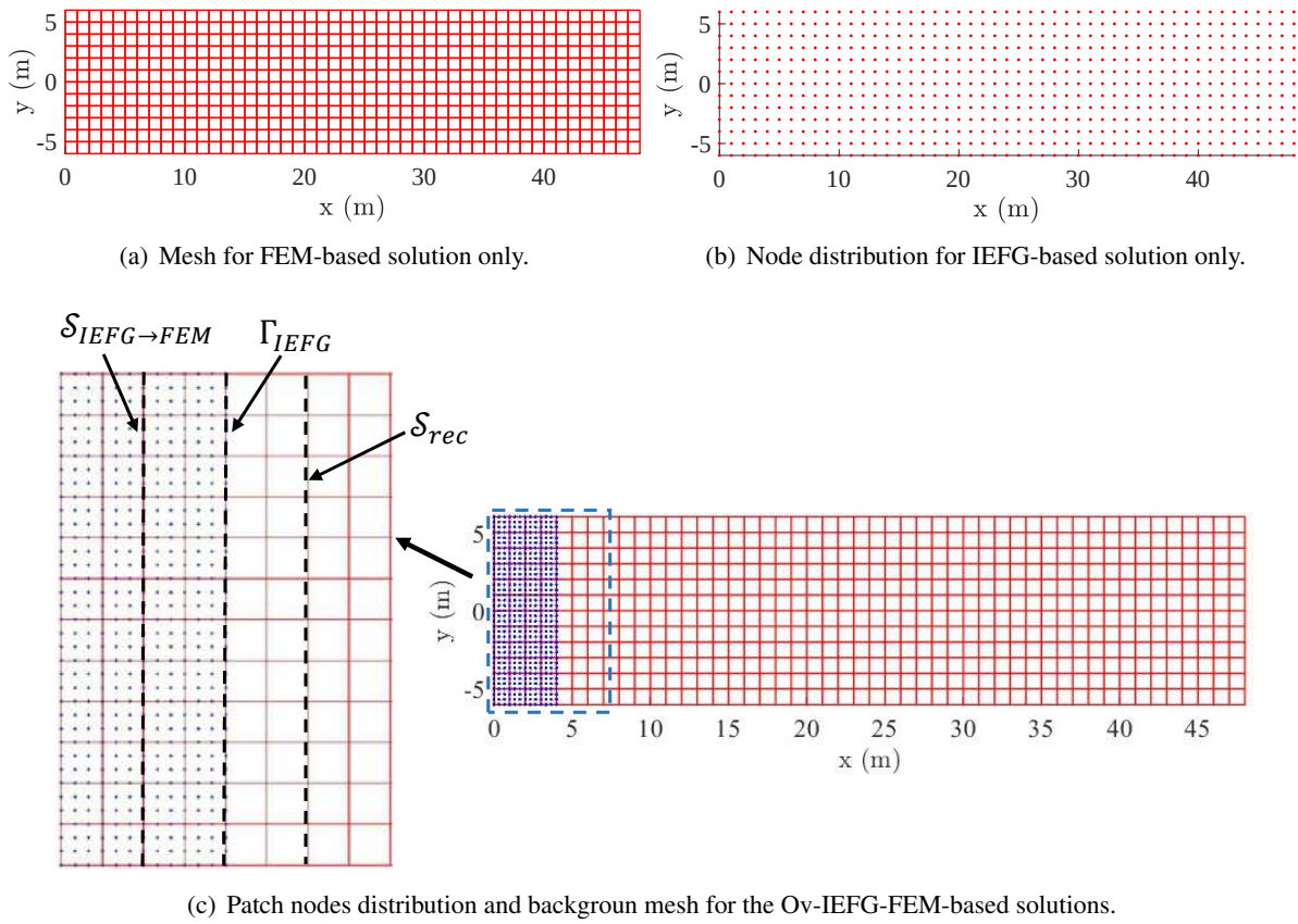
Figura F.3: Intermediate meshes and node distributions used in the cantilever beam analysis via (a) FEM, (b) IEFG, and (c) Ov-IEFG-FEM. For the Ov-IEFG-FEM, the patch of nodes and background mesh are depicted in blue and red, respectively. Black dashed lines are used to indicate the immersed contours \mathcal{S}_{IEFG \rightarrow FEM} , \mathcal{S}_{rec} , and also the boundary \Gamma_{IEFG} of the patch domain \Omega_{IEFG} . The displacements \tilde{U}_{FEM} are imposed on \Gamma_{IEFG} by integration via the penalty method, whereas \tilde{U}_{FEM} are imposed at nodes h \in \mathcal{N}_{enc} enclosed by \mathcal{S}_{IEFG \rightarrow FEM} .
