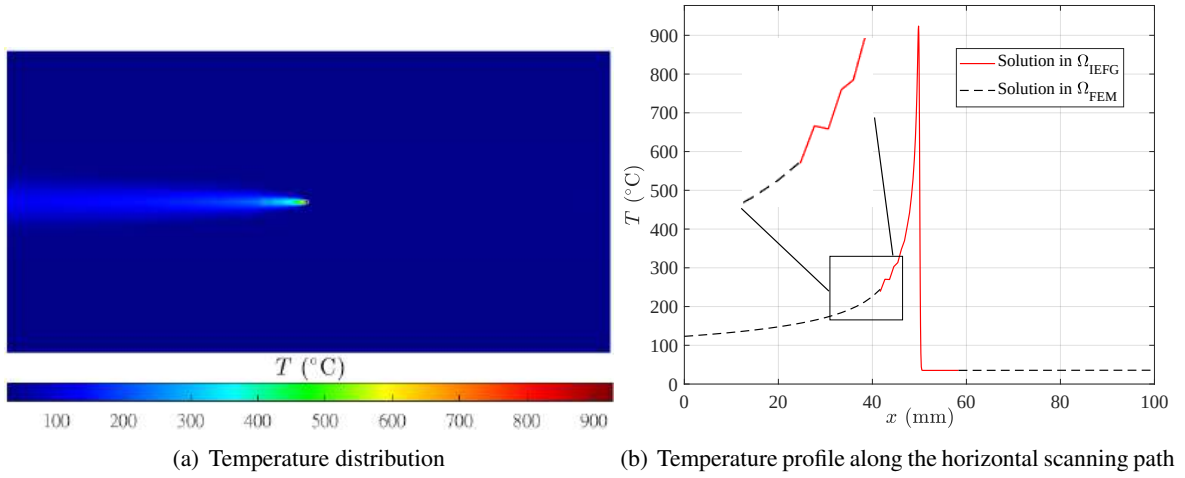
Figure E.28: Unstable results obtained via the Ov-IEFG-FEM with advection dominating the heat transfer problem in the moving domain \Omega_{IEFG} , when it is solved under a standard Bunov-Galerkin formulation. These results correspond to t = 0.5 s.
