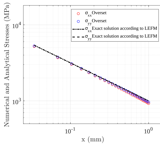
Figura F.17: Comparison of the numerical solutions obtained via the Ov-IEFG-FEM with the reference solution developed by Tada[1]
