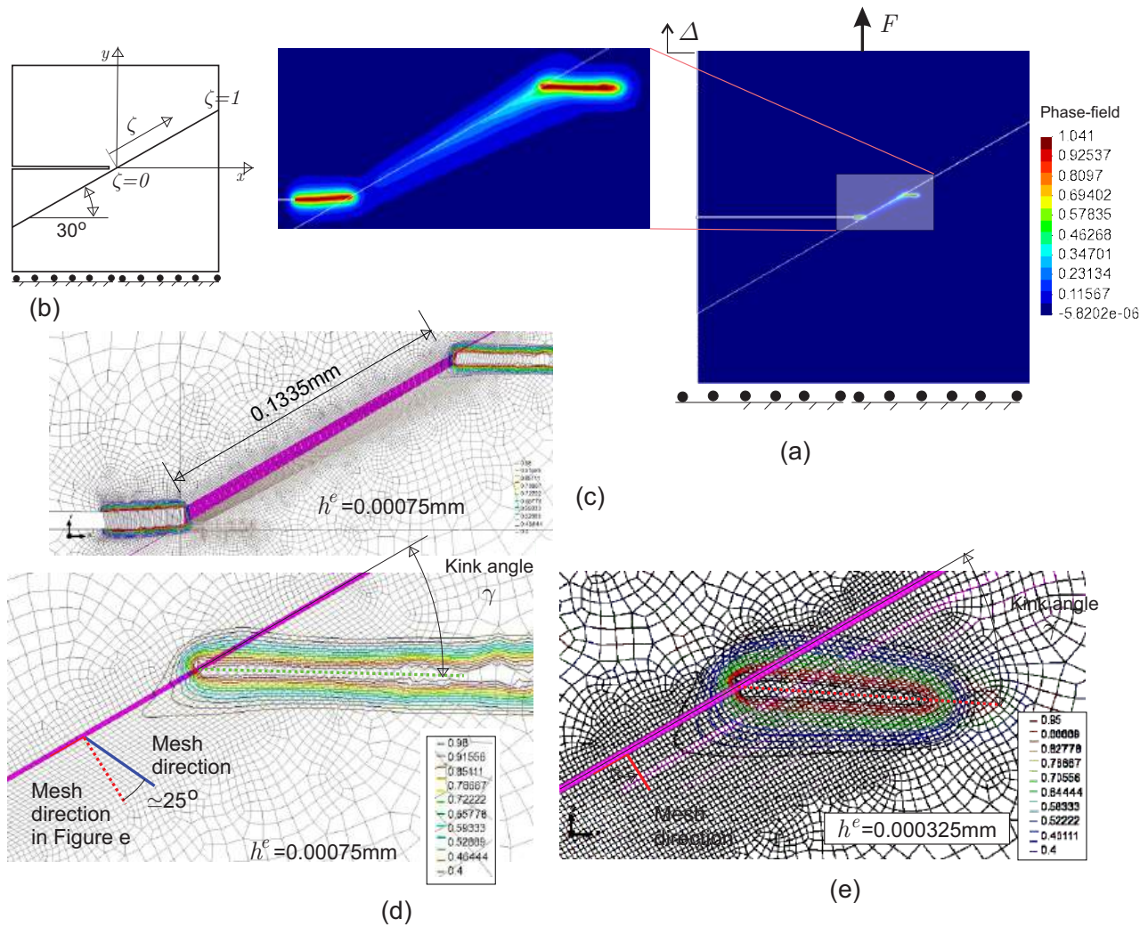
Figura A.10: Analysis of a crack kinking out of an interface. a) Iso-maps of phase-field at the end of analysis. b) The interface parameters changes with the coordinates \zeta . c-d) Deformed mesh and phase-field iso-curves, mesh with h^e = 7.5 \times 10^{-4}\text{mm} . e) Phase-field iso-curves, mesh with h^e = 3.25 \times 10^{-4}\text{mm} .
