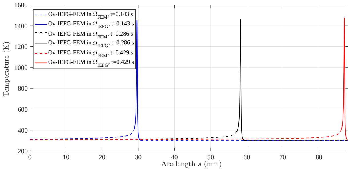
Figura E.23: Temperature profiles along the arc length s covered by the heat source path in the non-linear applied three-dimensional problem with curved geometry.
