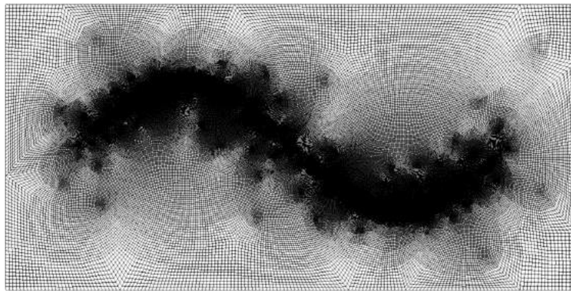
Figura E.14: Fine mesh for the FEM-based solution of the transient heat conduction problem over the rectangular thin plate with a moving heat source following a sinusoidal path. The mesh is very refined along the scanning path.
