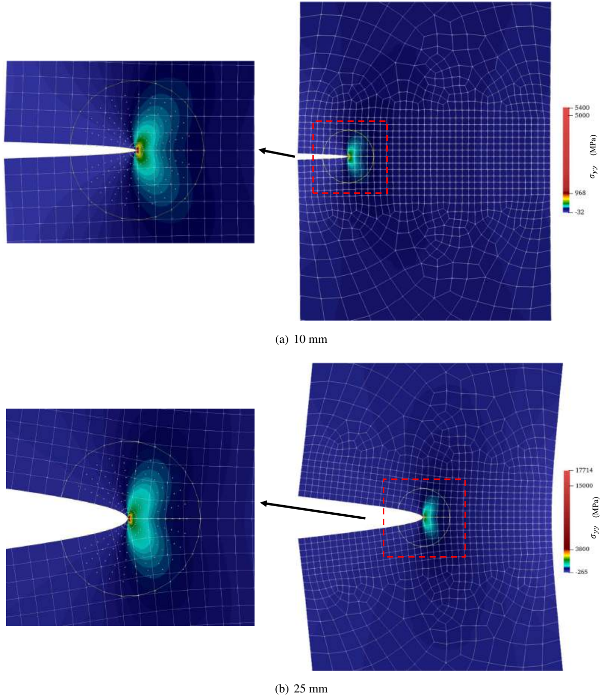
Figura F.18: \sigma_{yy} stress distribution for SENT specimen with structured background mesh for different crack lengths.
