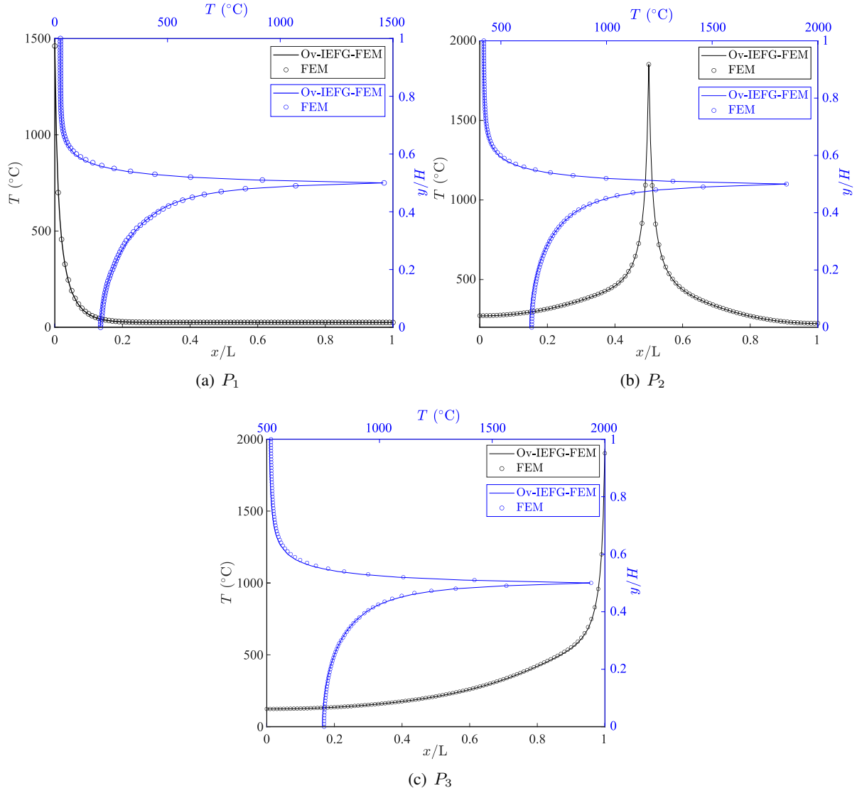
Figura E.19: Temperature profiles computed along the horizontal (black) and vertical (blue) axes passing over the current heat source position, comparison between the results computed via the proposed Ov-IEFG-FEM and a very fine FEM-based solution.
